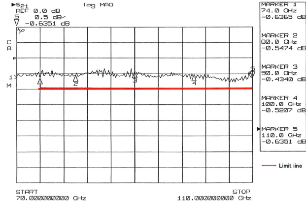
Insertion loss
