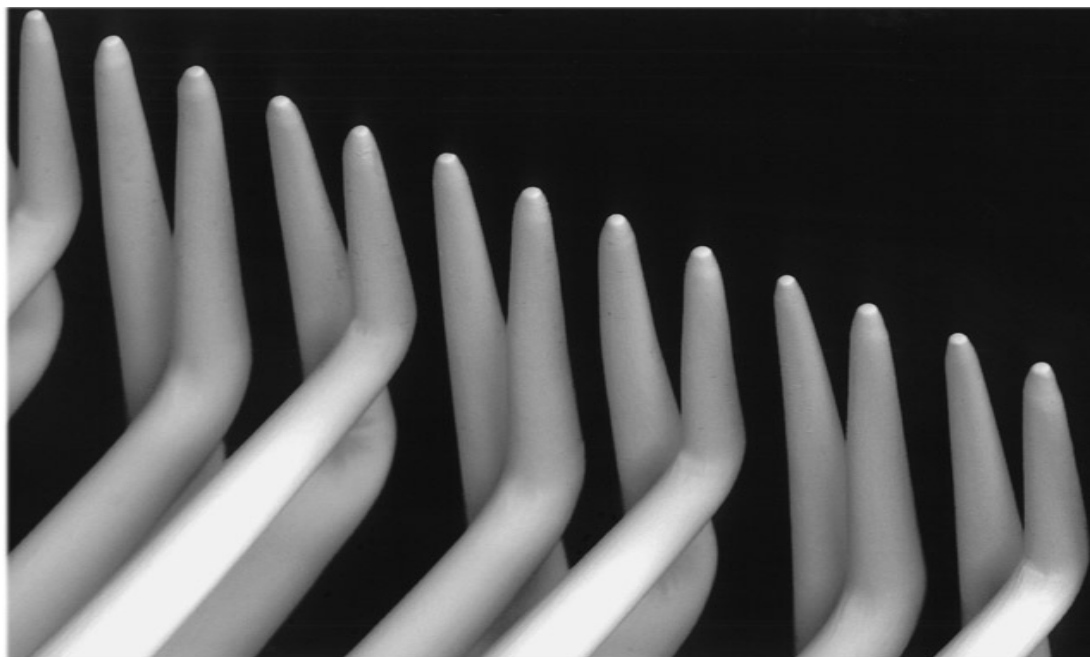
40 \mu m pitch for LCD Driver IC
